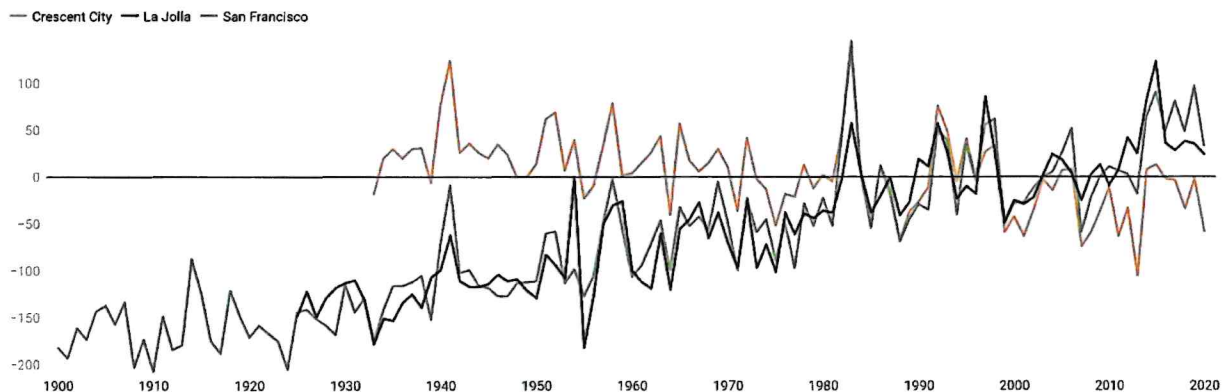
Figure 263: Annual Mean Sea Level Trends
