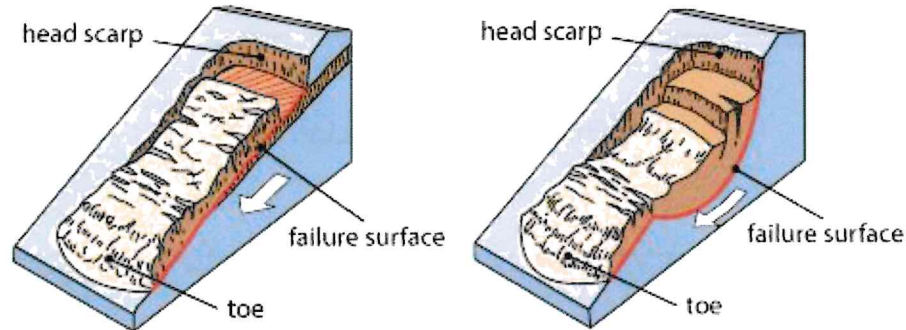
Figure 265: Mud Flow Areas
