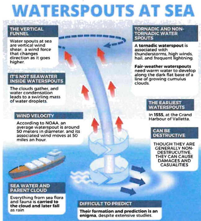
Figure 290: Waterspout Formation
