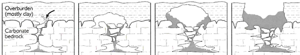
Figure 276: Cover-Collapse Sinkhole Formation
