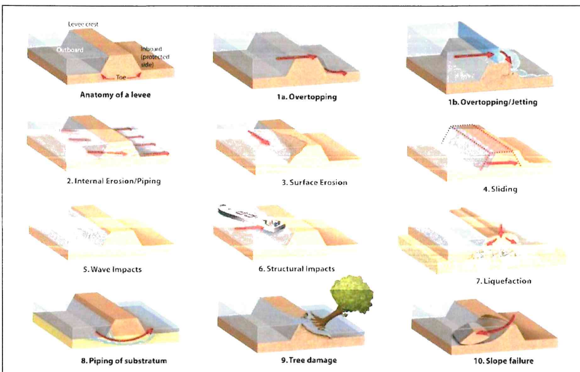
Figure 277: Levee Failure Mechanisms
