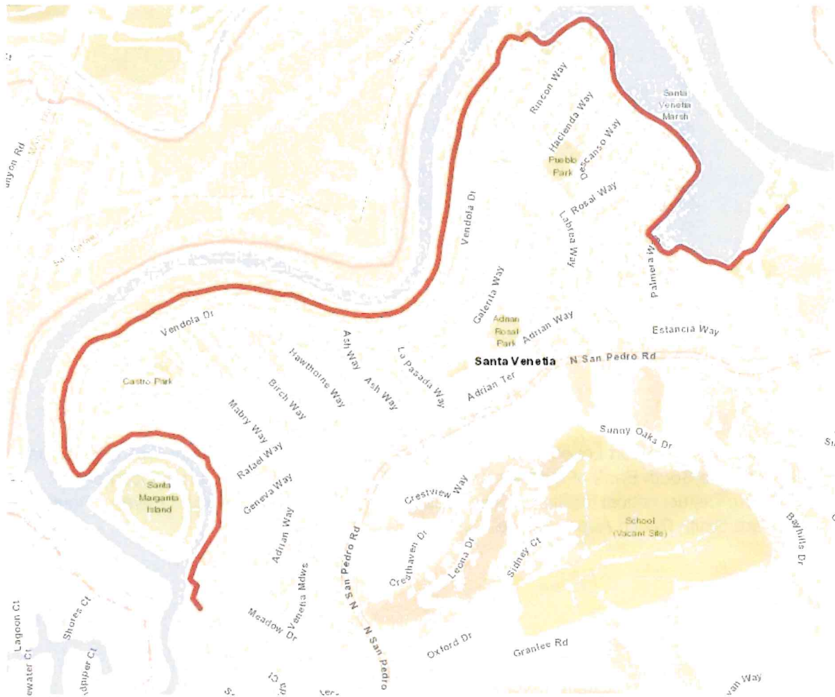
Figure 280: Santa Venetia Levee in Santa Venetia Source: U.S. Army Corps of Engineers
