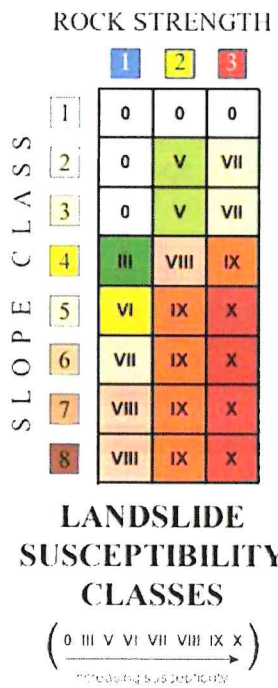
Figure 264: Landslide Susceptibility Classes Source: USGS
