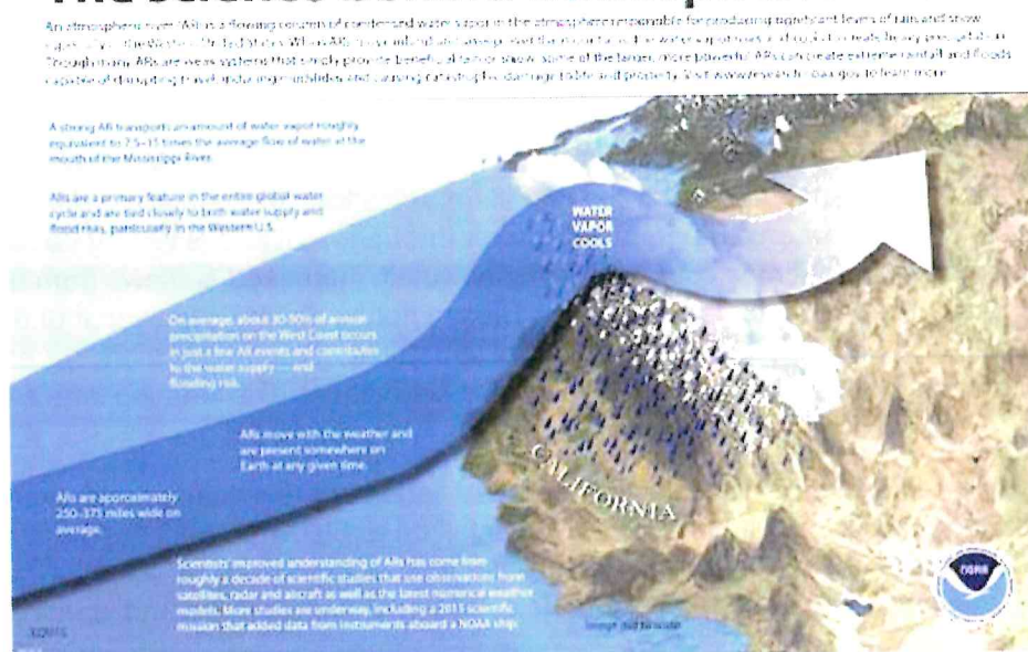
Figure 272: Diagram of an Atmospheric River Event Source: NOAA
