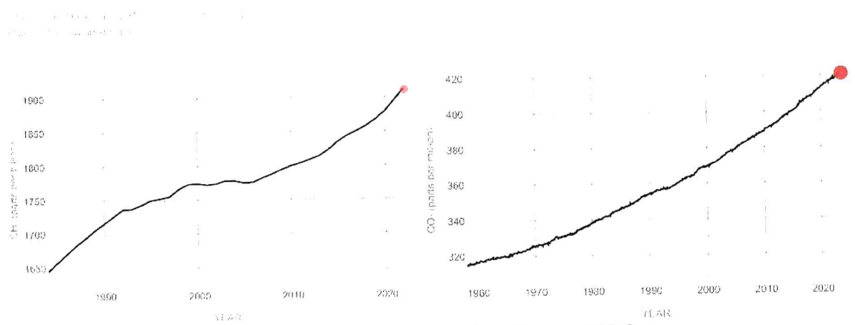
Figure 260: NASA Global Temperature Change CO2 Gas Source: NASA Global Climate Change, 2022
