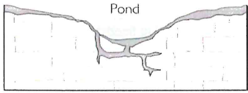
Figure 274: Dissolution Sinkhole Formation Source: USGS
