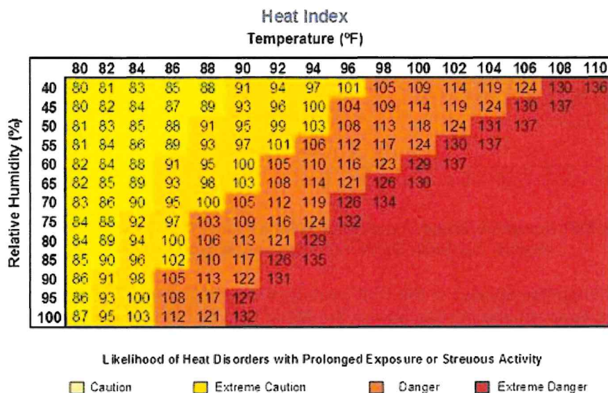
Figure 286: Heat Index Source: NOAA
