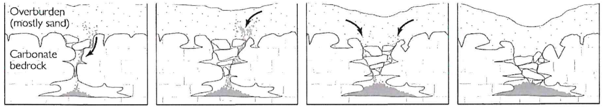
Figure 275: Cover-Subsidence Sinkhole Formation Source: USGS
