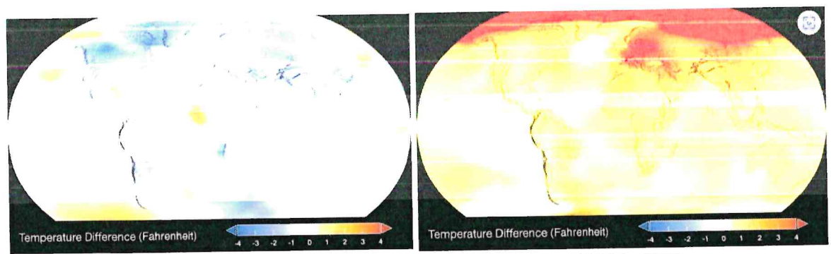
Figure 261: NASA Global Temperature Change 1884 to 2022 Source: NASA Global Climate Change, 2022
